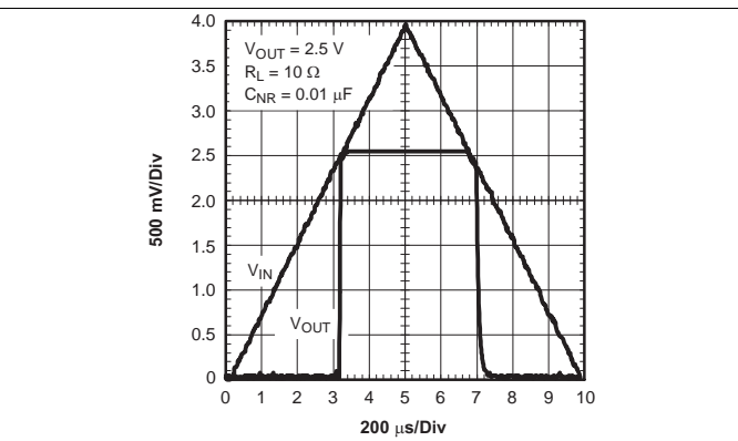
Figure 14. TPS79630 Line Transient Response
