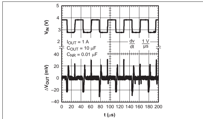
Figure 13. TPS79618 Line Transient Response
